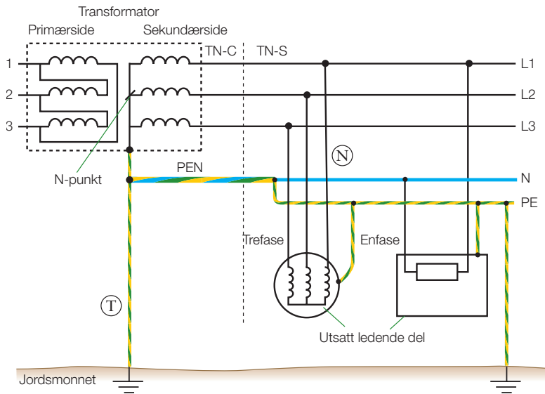
Figur 10.3 Prinsippskisse for TN-system
