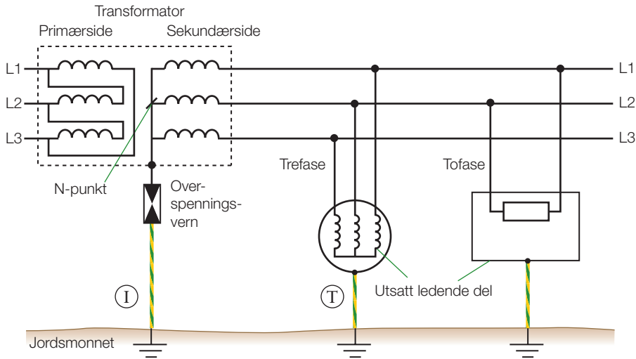
Figur 10.2 Prinsippskisse for IT-system
